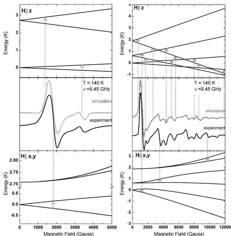
Figure 3. Experimentally observed and simulated spectra of 2 (left) and 3 (right) with the energy-level diagram for the principal symmetry axis, H \parallel Z , and the perpendicular X,Y directions. The arrows mark the EPR transition assignments.
